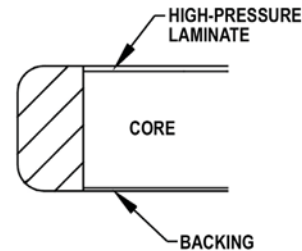
Matrix Series Flush Edge
