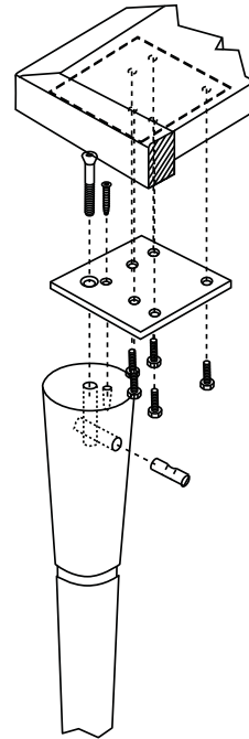
Matrix Series Wood Leg
