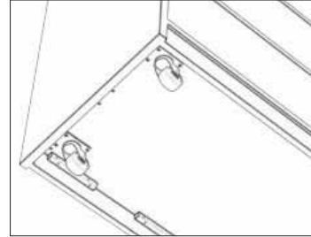
Bottom Caster View
