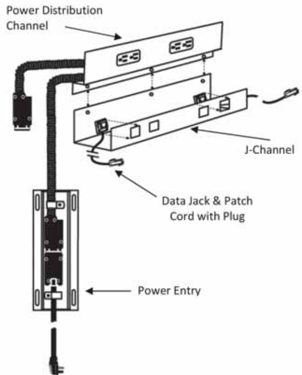
Panel Wire Manager Assembly for Data and Power
