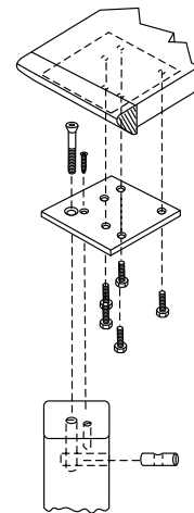
Chancellor's Series Leg Without Apron
