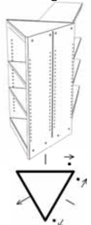
Transitional Tower Adders, Type 3 Double- to Single-Faced
